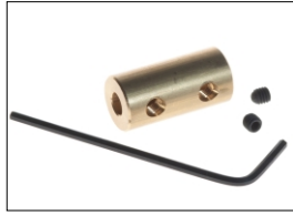
Part No. 919D1/2. In-line Coupling. 6mm-8mm (Meccano) Dia. 10mm x 20mm. 23g
