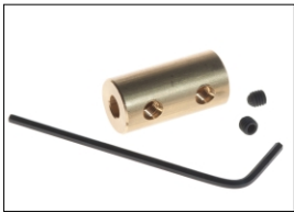
Part No. 919D1. In-Line Coupling. 6mm - 6mm. (Dia. 12.67mm x 24.8mm). 23g
